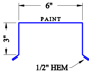
HW-22 COPING
