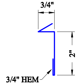
HW-25 COUNTER FLASHING
