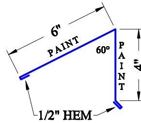
HW-18 MONO-SLOPE RIDGE CAP
