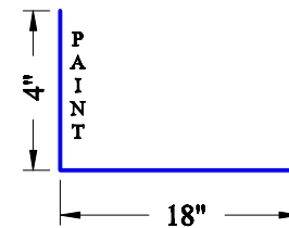
HW-24 CHIMNEY FLASHING (TS)
